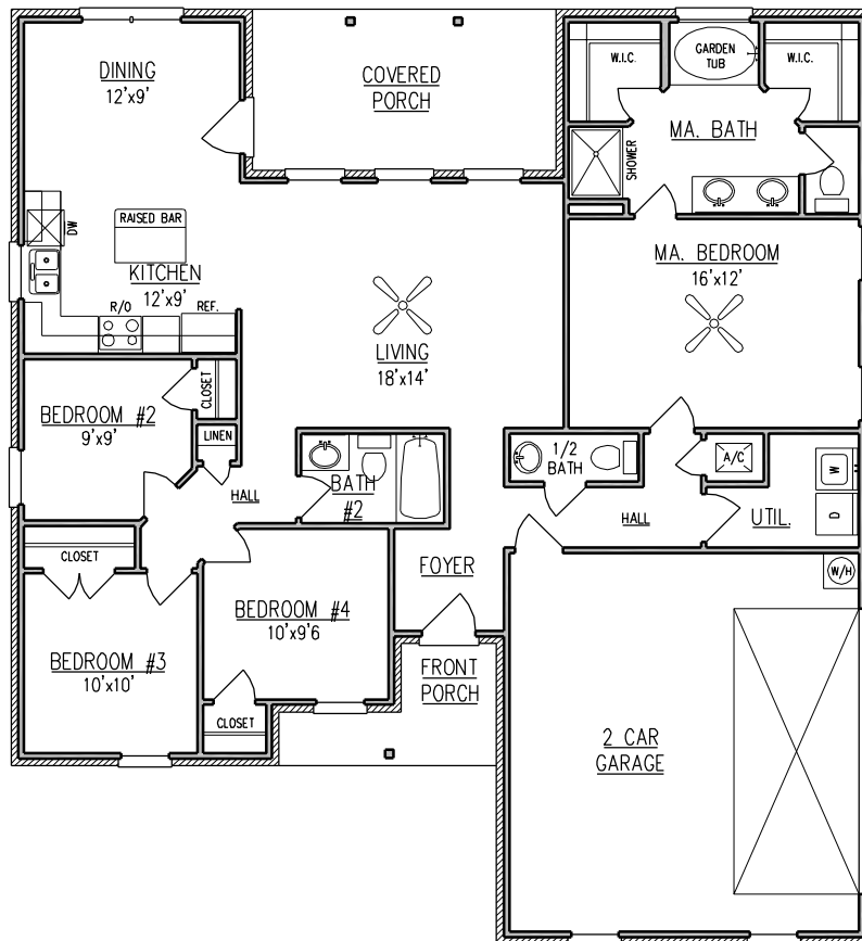
FLOOR PLAN
