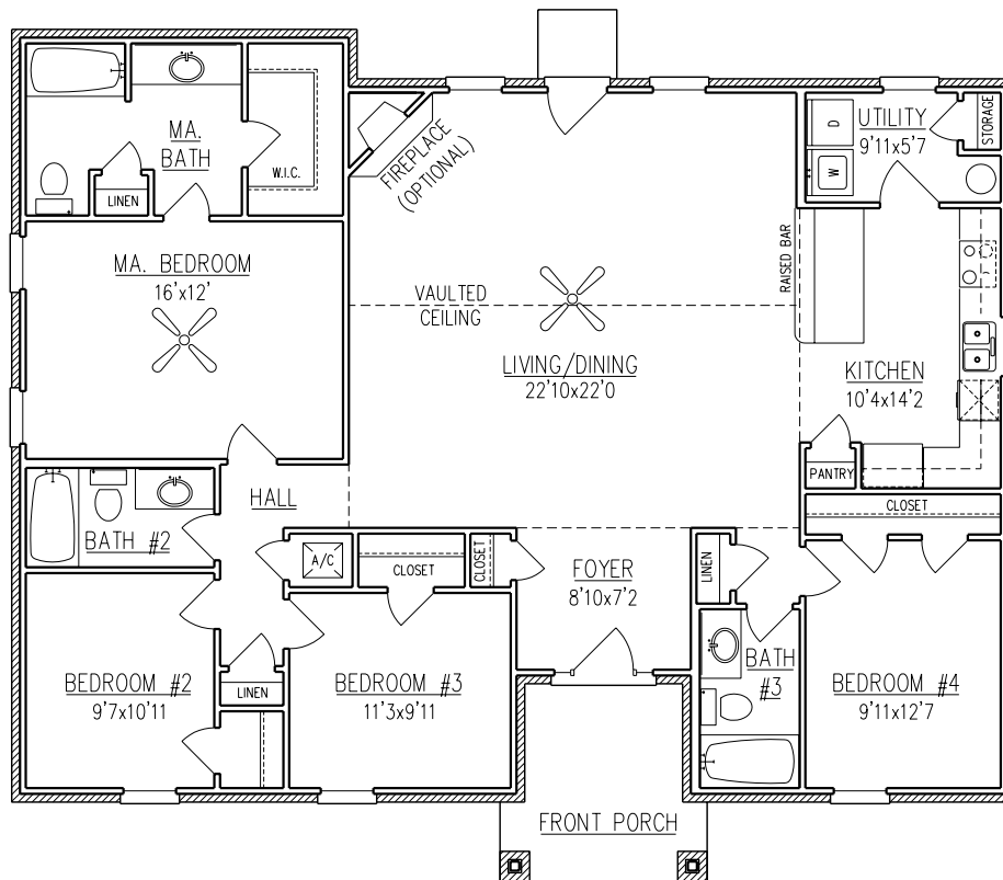
FLOOR PLAN
