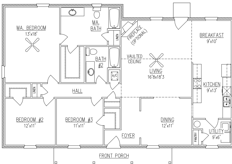
FLOOR PLAN
