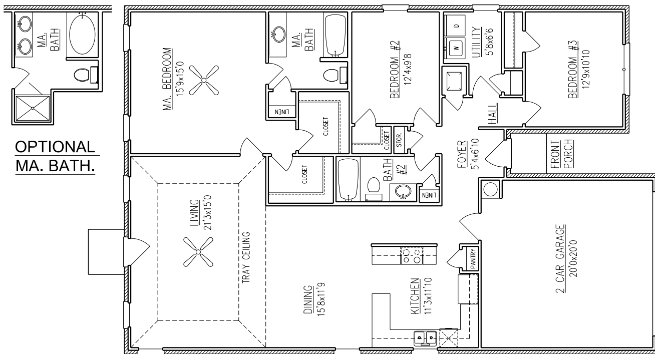
FLOOR PLAN
